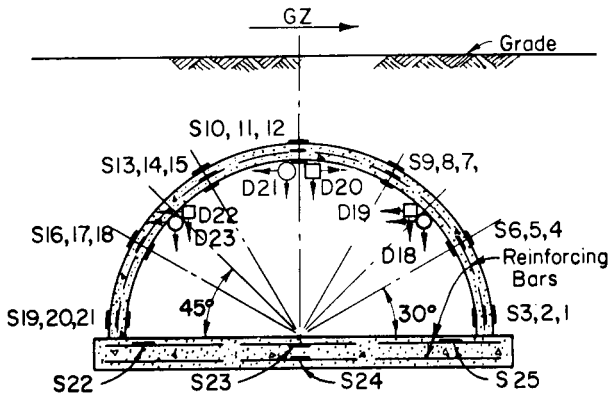
SECTION F-F
